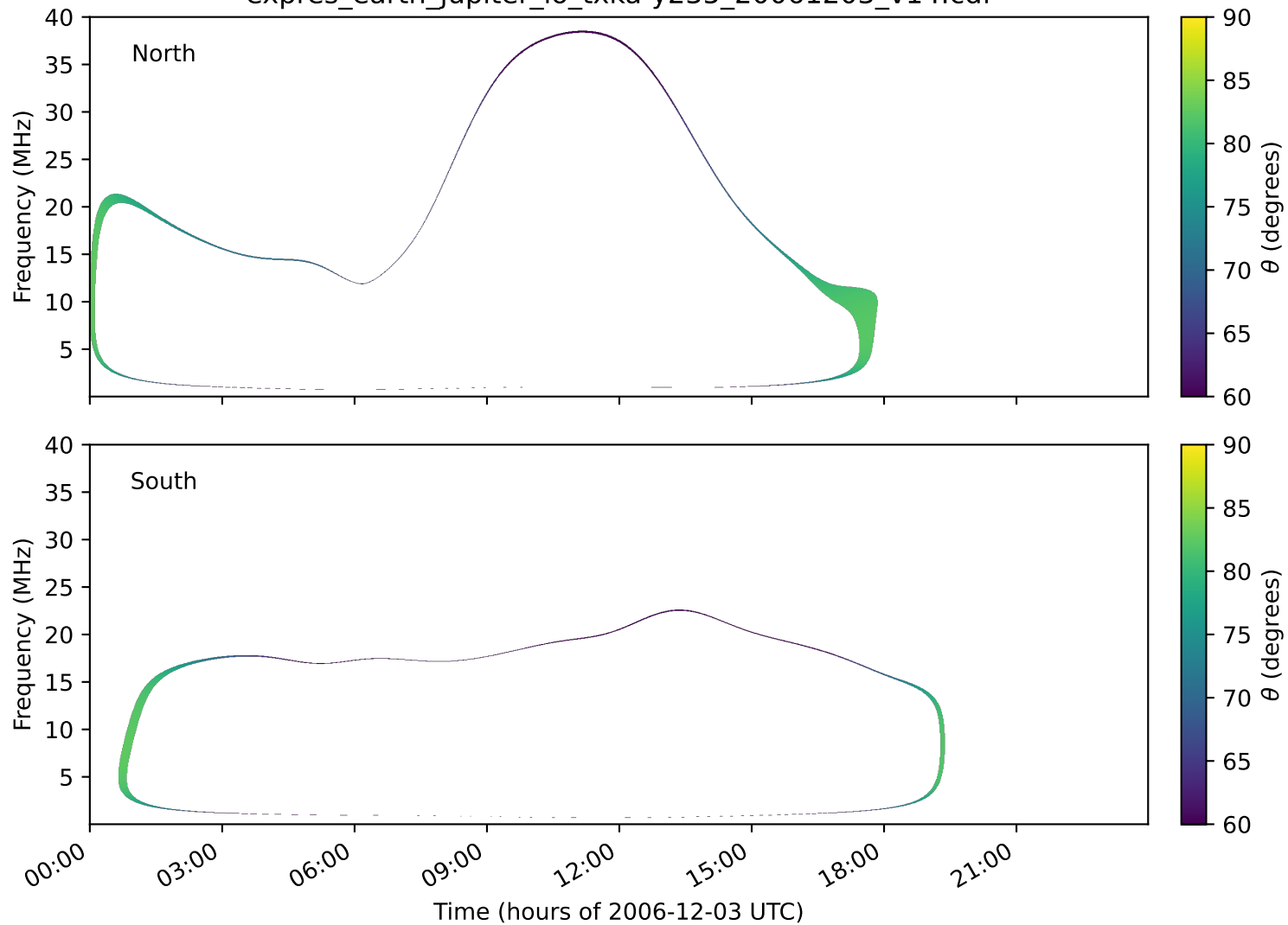
expres_earth_jupiter_io_txka-y235_20061203_v14.cdf
