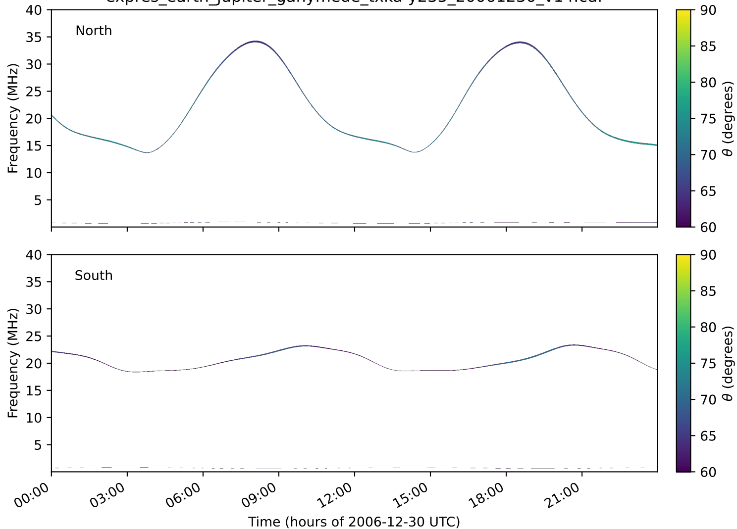
expres_earth_jupiter_ganymede_txka-y235_20061230_v14.cdf
