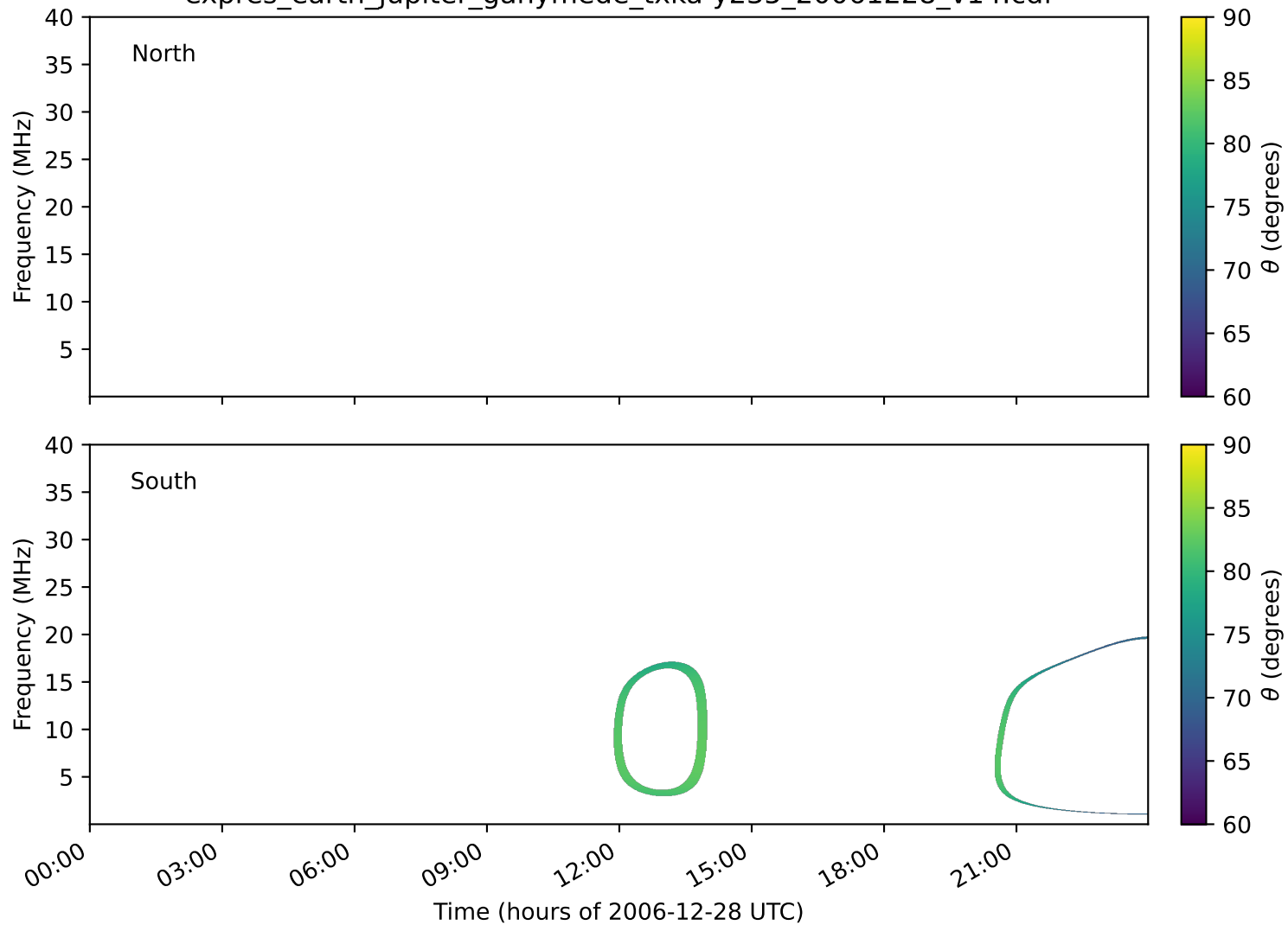
expres_earth_jupiter_ganymede_txka-y235_20061228_v14.cdf
