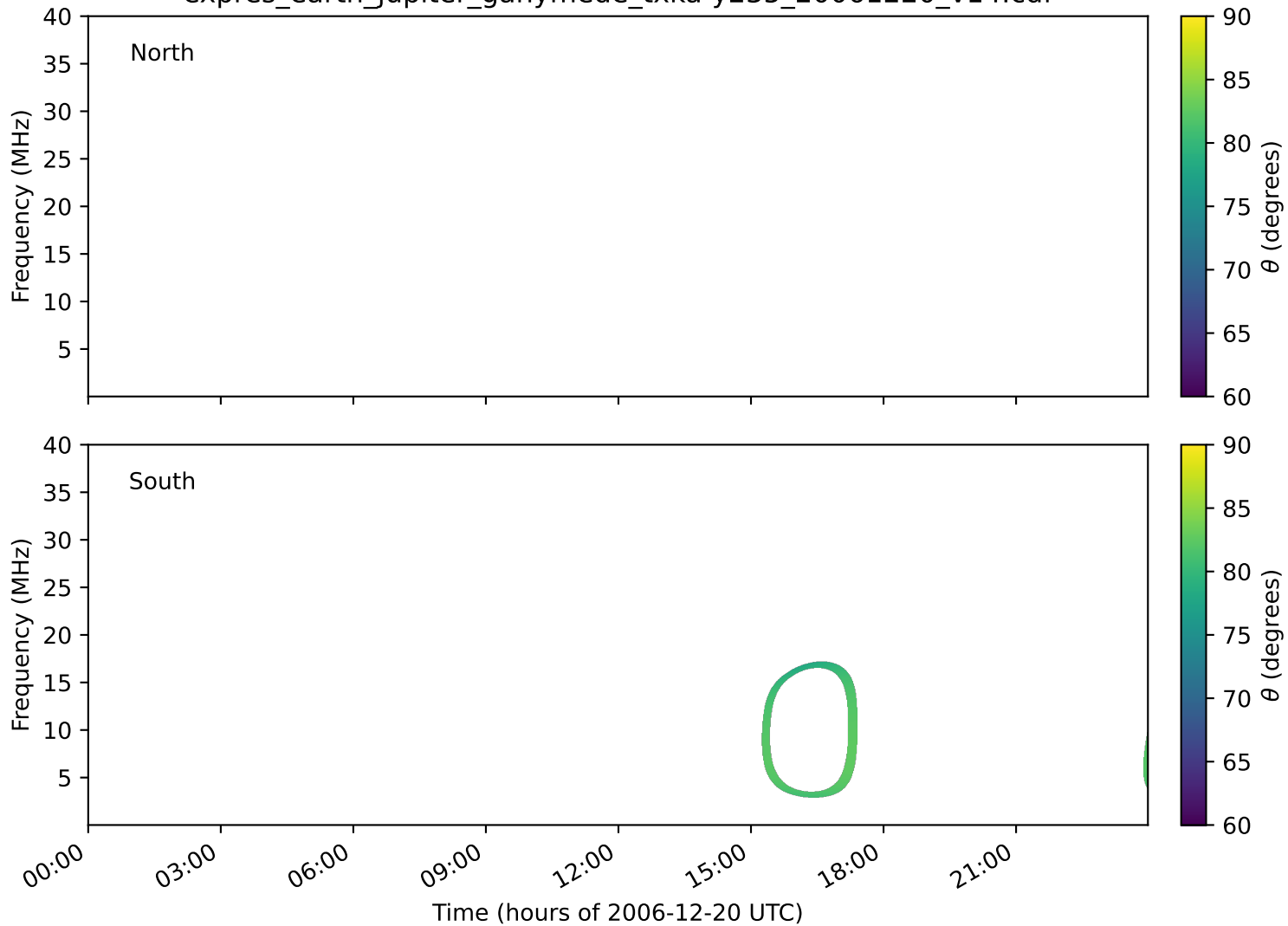
expres_earth_jupiter_ganymede_txka-y235_20061220_v14.cdf
