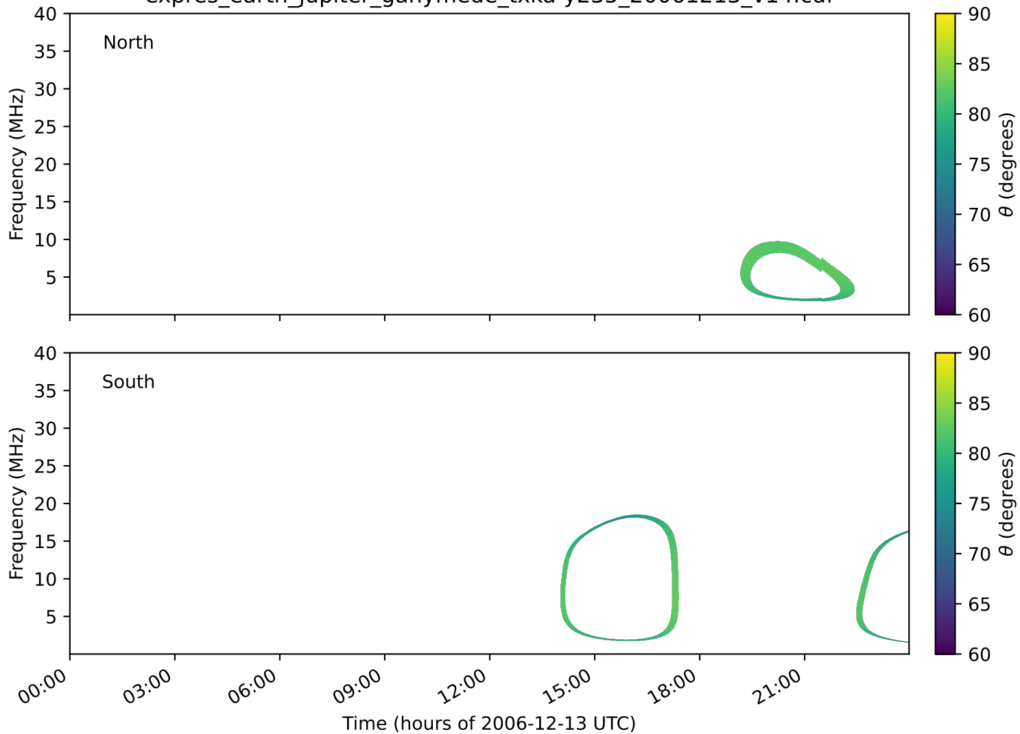
expres_earth_jupiter_ganymede_txka-y235_20061213_v14.cdf
