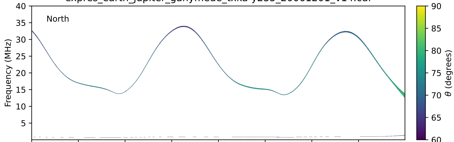
expres_earth_jupiter_ganymede_txka-y235_20061201_v14.cdf
