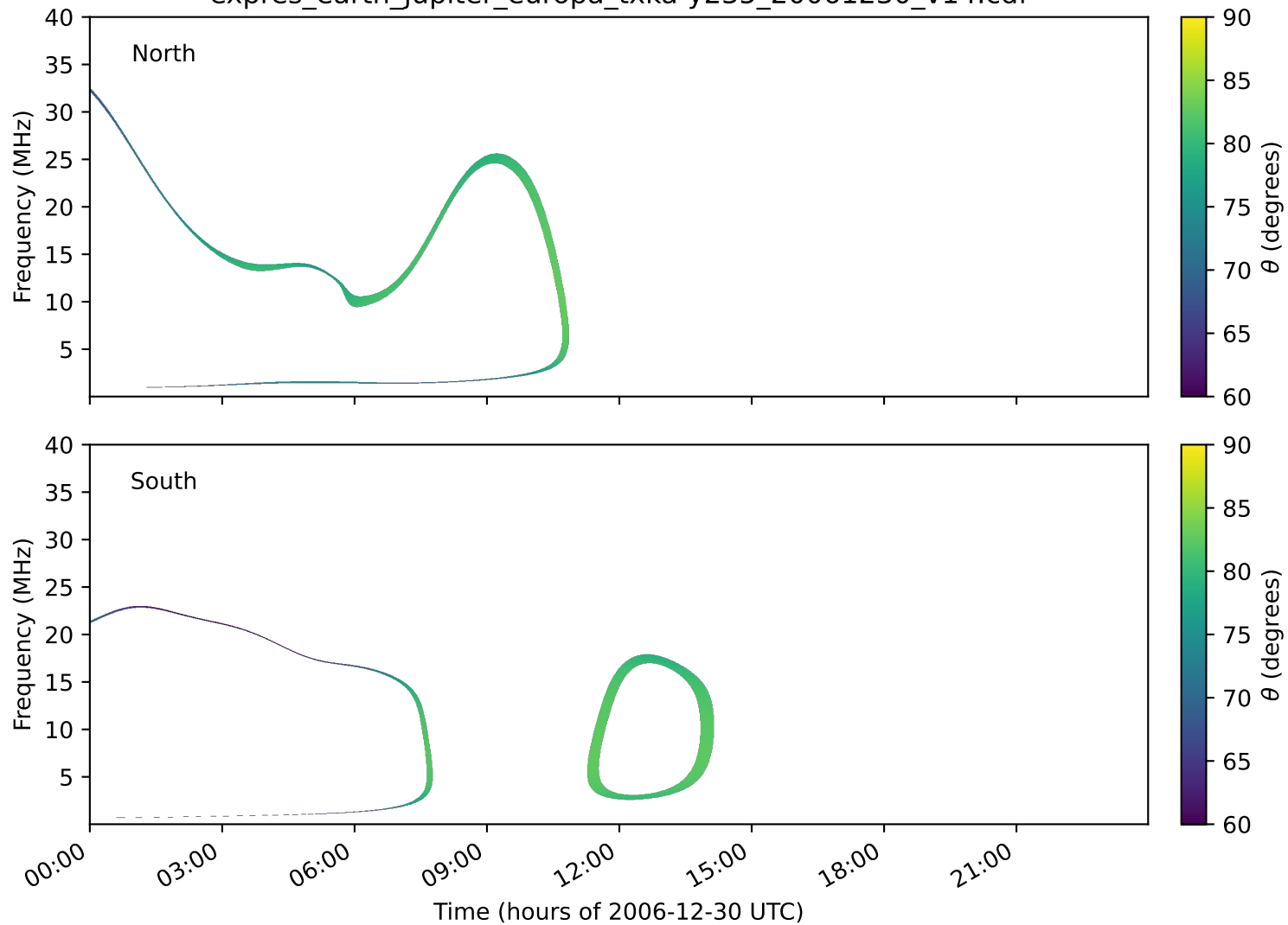
expres_earth_jupiter_europa_txka-y235_20061230_v14.cdf
