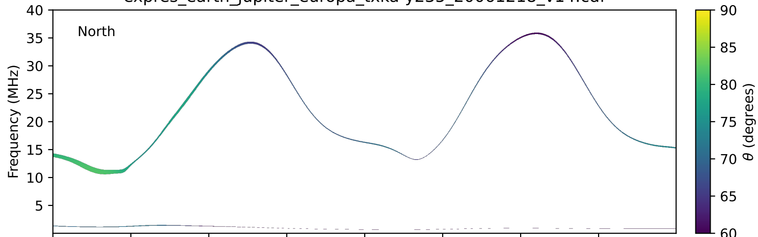
expres_earth_jupiter_europa_txka-y235_20061218_v14.cdf
