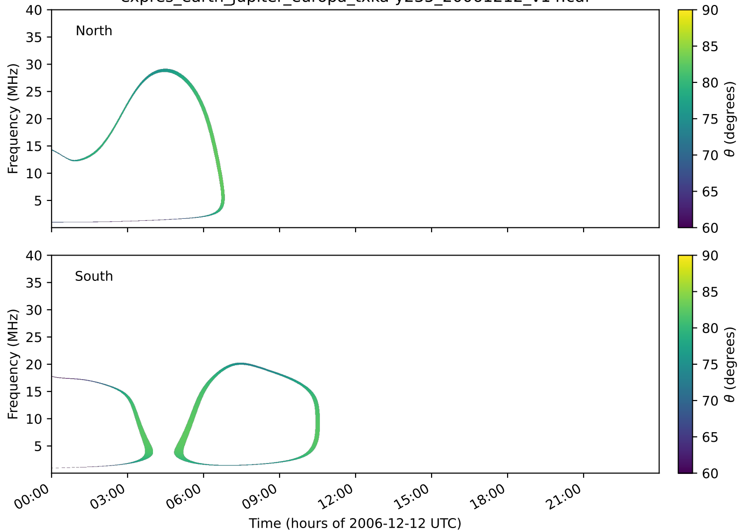
expres_earth_jupiter_europa_txka-y235_20061212_v14.cdf
