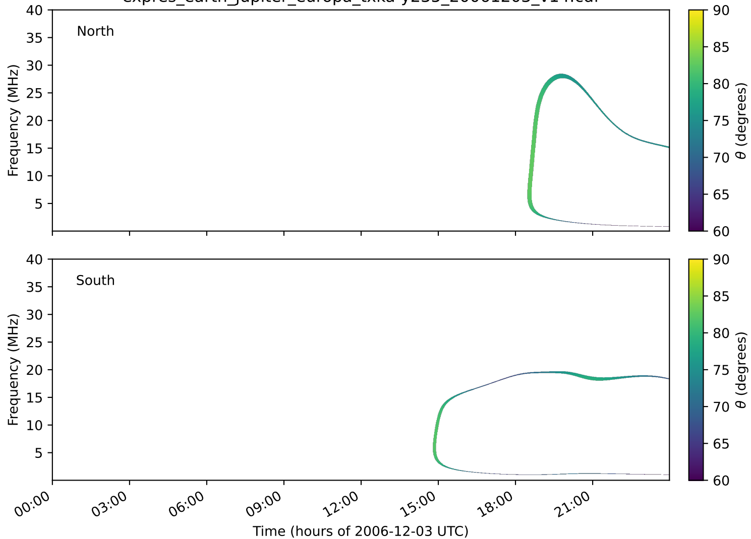
expres_earth_jupiter_europa_txka-y235_20061203_v14.cdf
