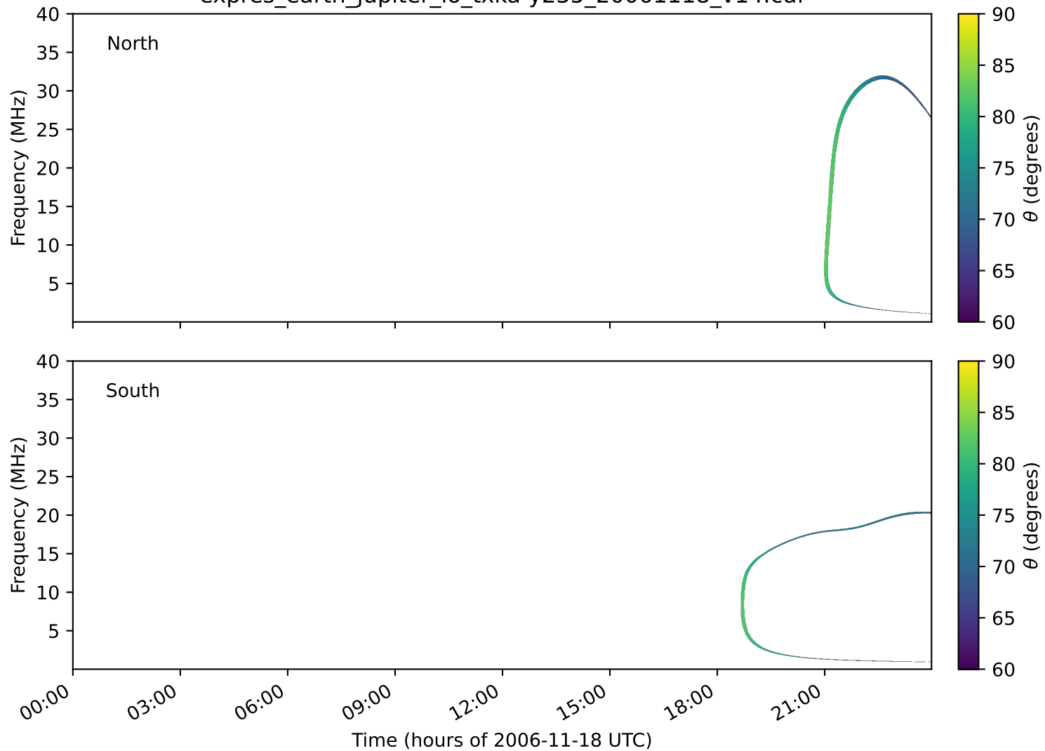
expres_earth_jupiter_io_txka-y235_20061118_v14.cdf
