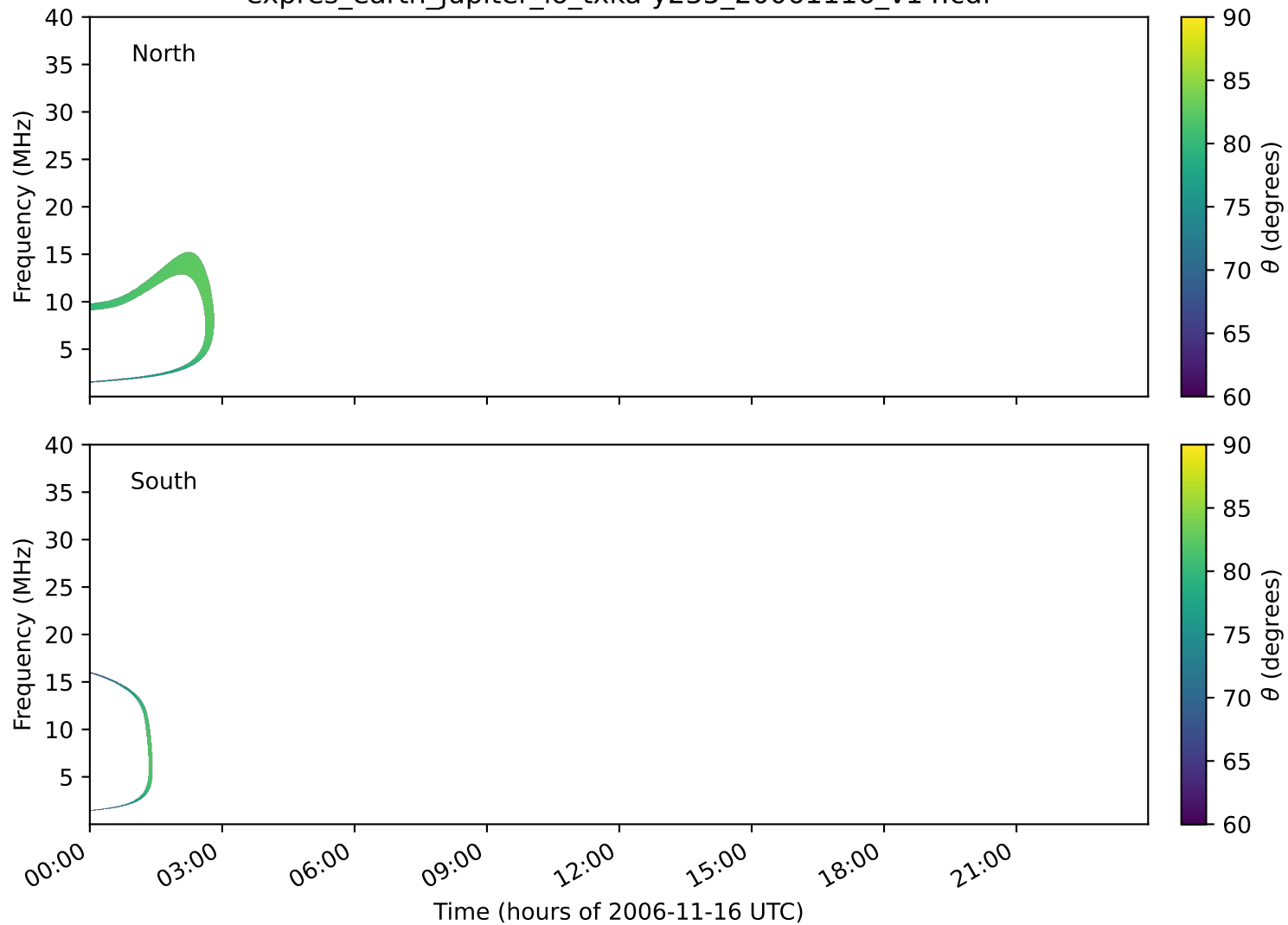
expres_earth_jupiter_io_txka-y235_20061116_v14.cdf
