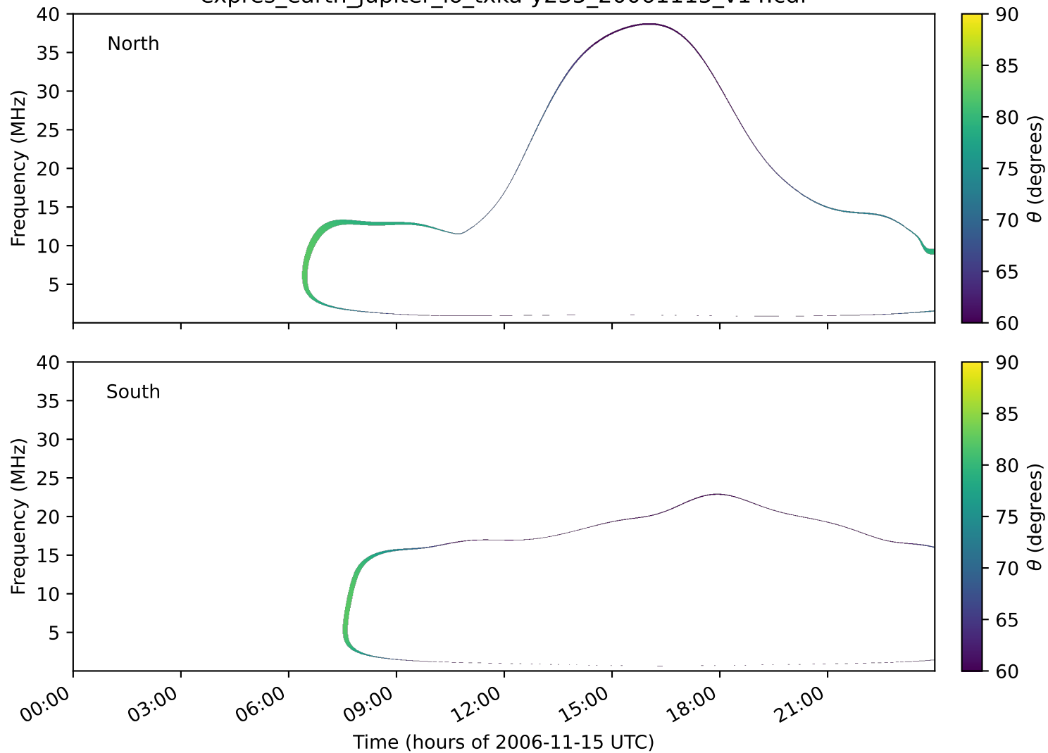
expres_earth_jupiter_io_txka-y235_20061115_v14.cdf
