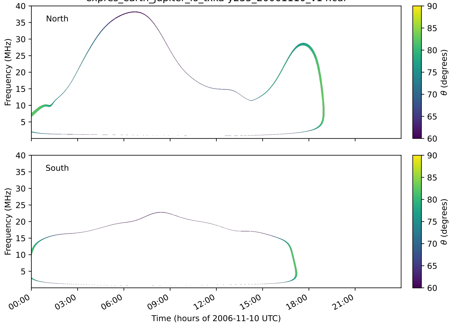
expres_earth_jupiter_io_txka-y235_20061110_v14.cdf
