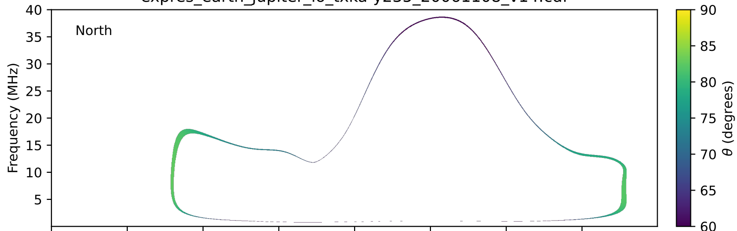
expres_earth_jupiter_io_txka-y235_20061108_v14.cdf
