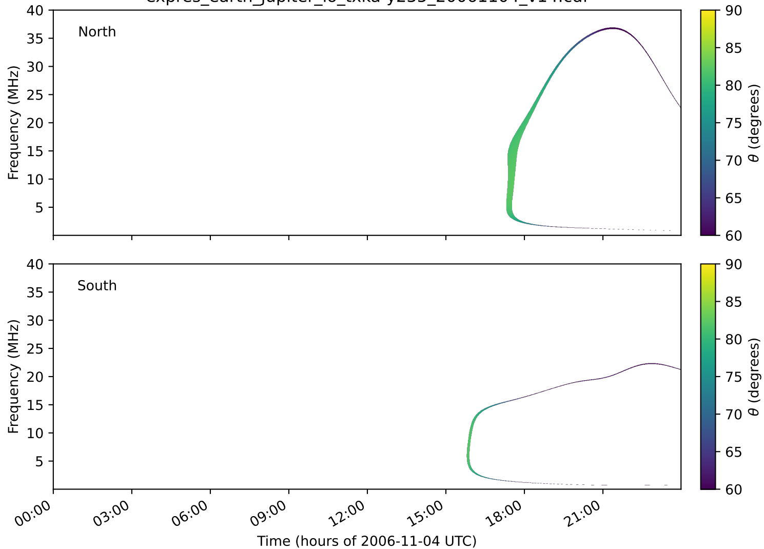
expres_earth_jupiter_io_txka-y235_20061104_v14.cdf
