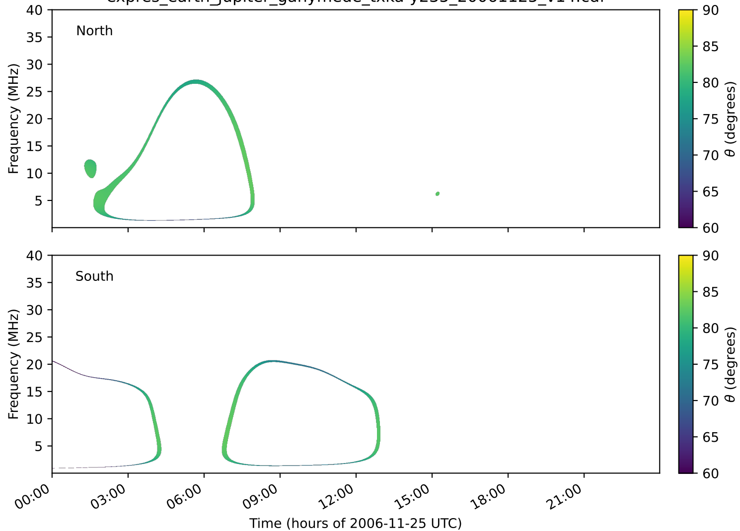
expres_earth_jupiter_ganymede_txka-y235_20061125_v14.cdf
