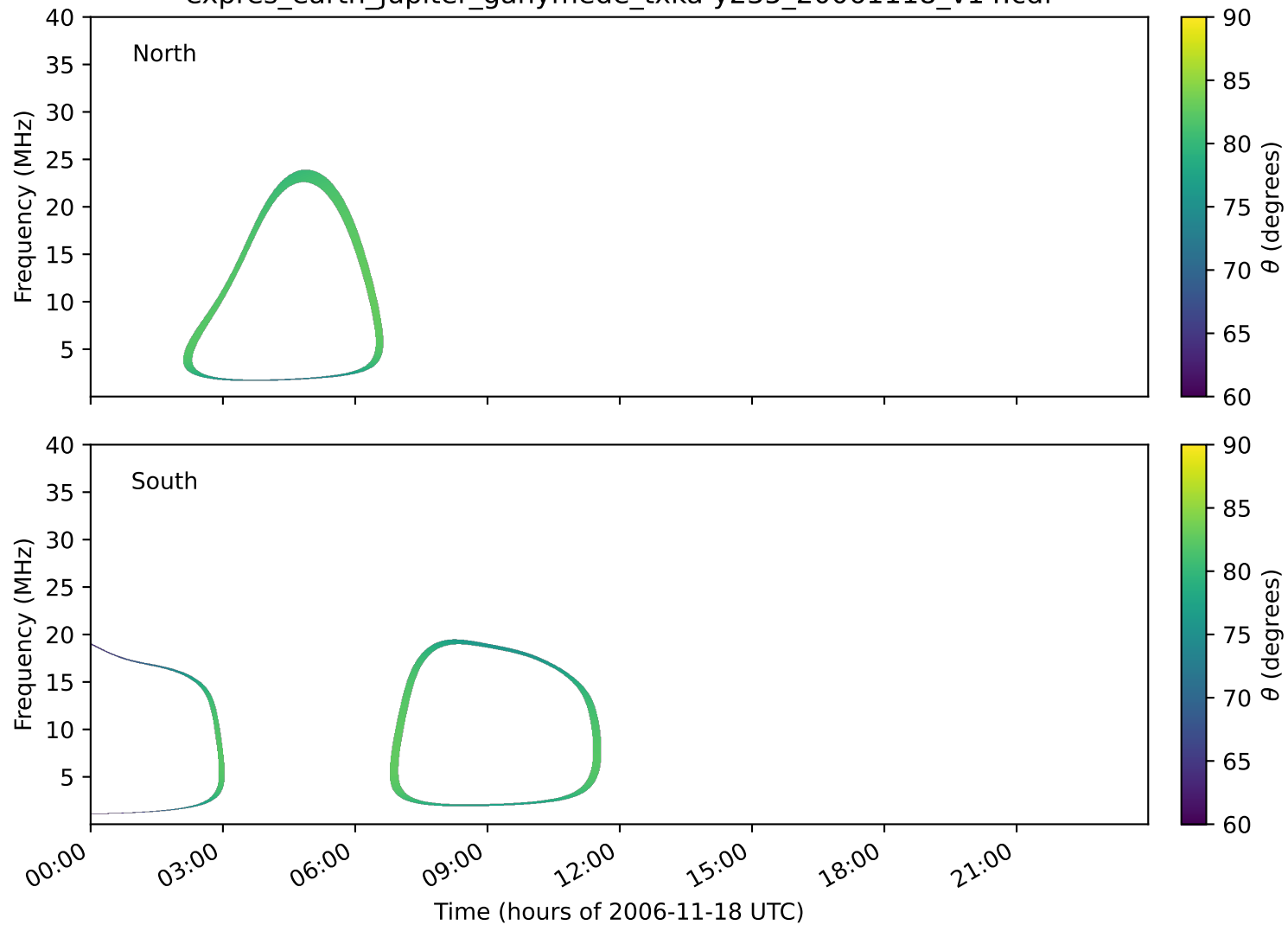
expres_earth_jupiter_ganymede_txka-y235_20061118_v14.cdf
