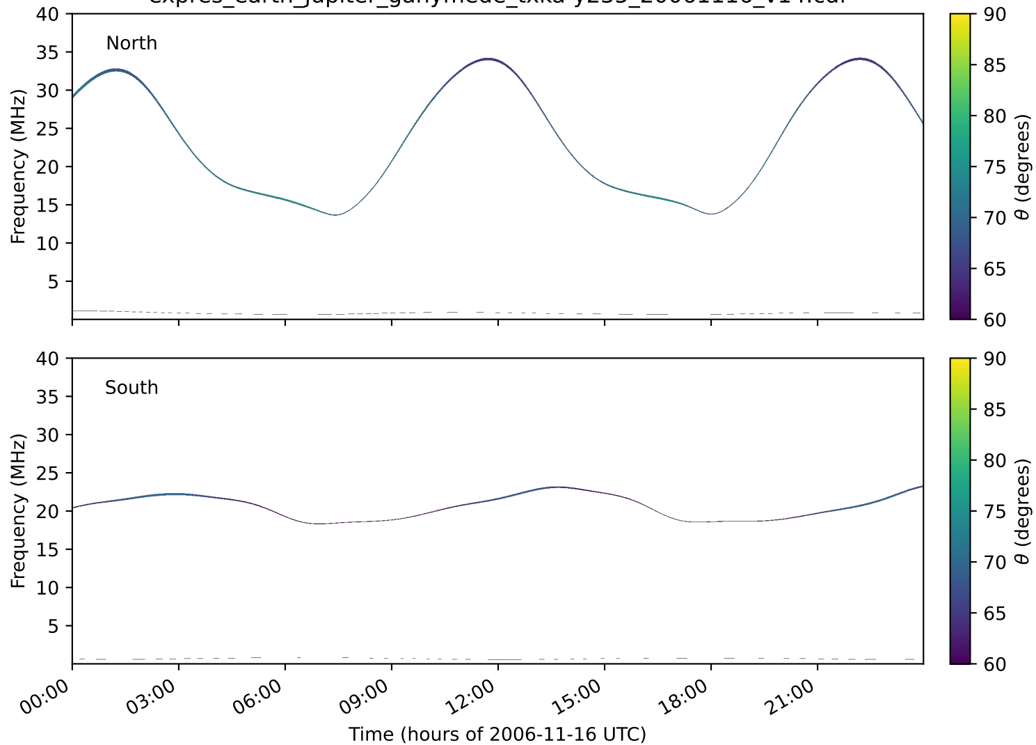
expres_earth_jupiter_ganymede_txka-y235_20061116_v14.cdf
