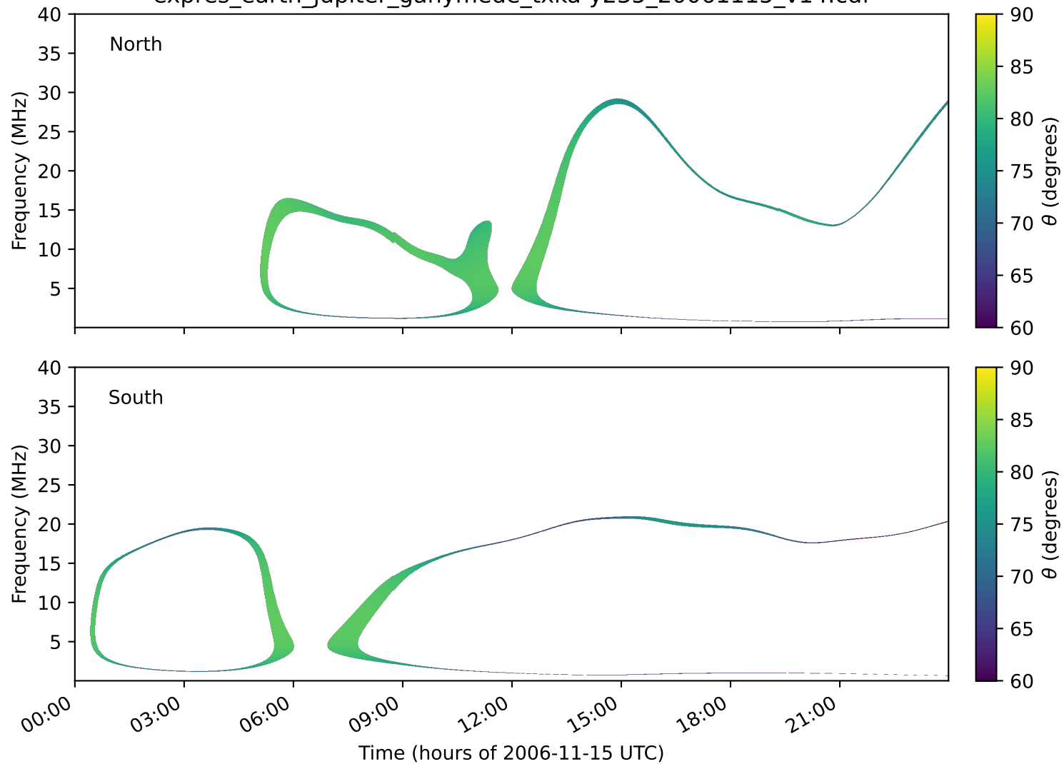
expres_earth_jupiter_ganymede_txka-y235_20061115_v14.cdf
