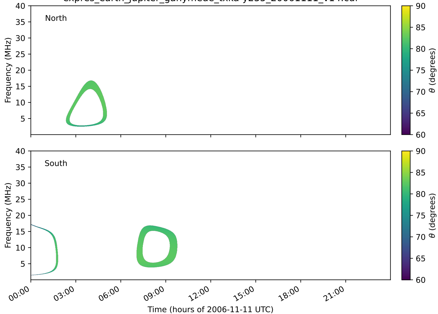
expres_earth_jupiter_ganymede_txka-y235_20061111_v14.cdf
