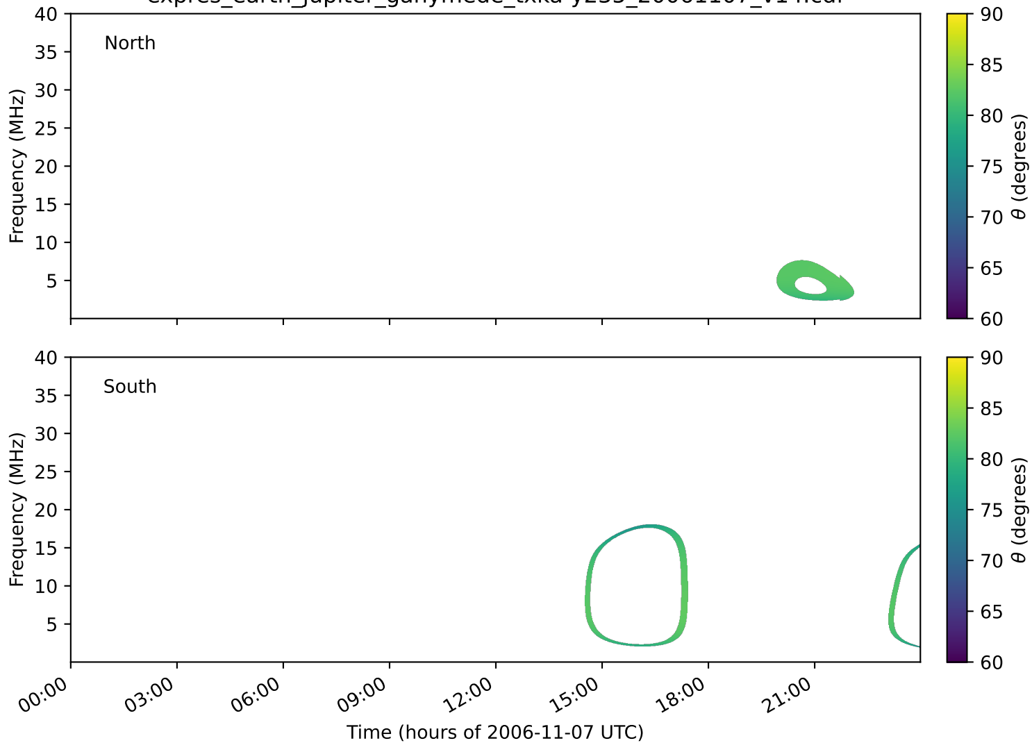
expres_earth_jupiter_ganymede_txka-y235_20061107_v14.cdf
