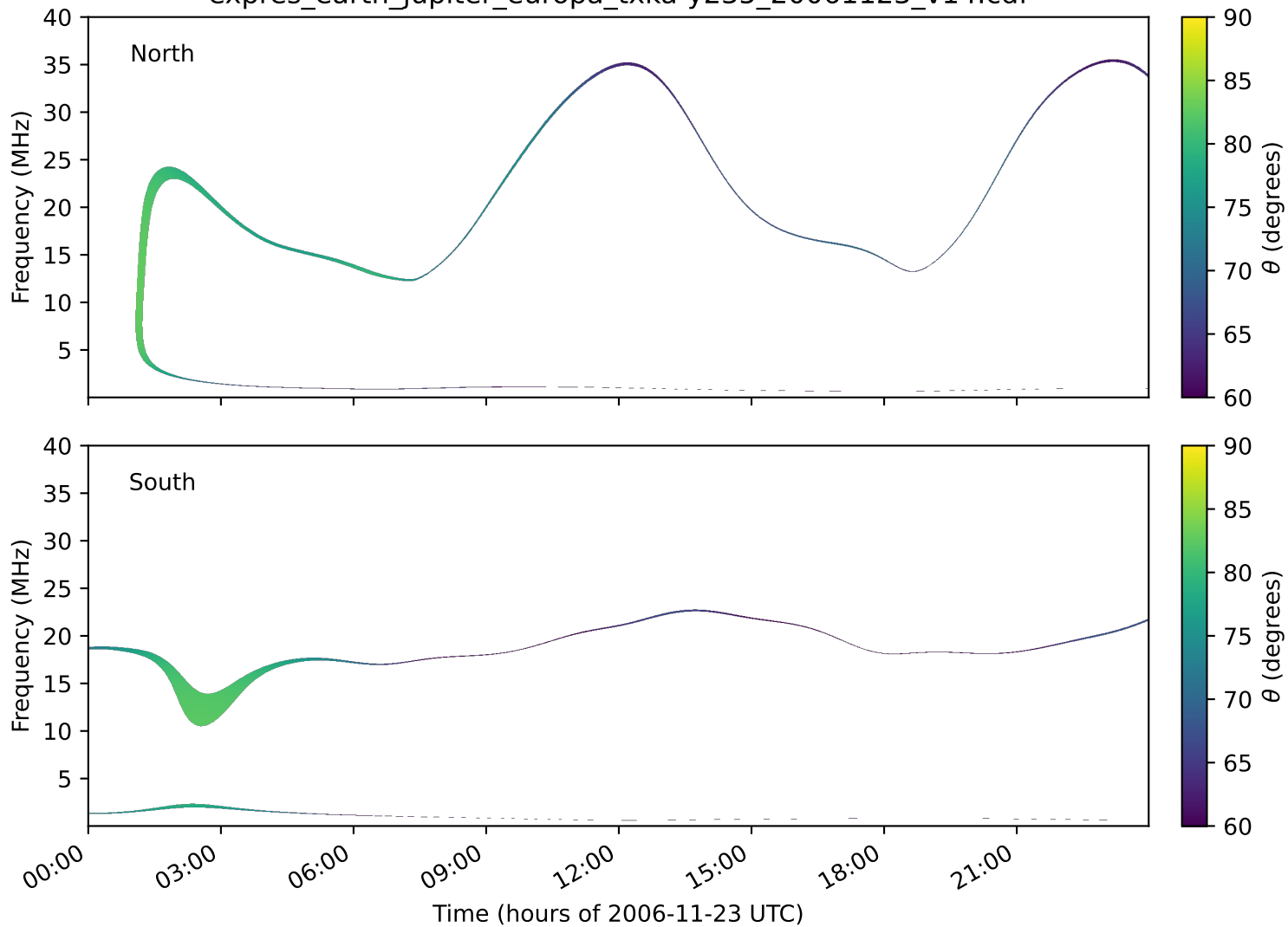
expres_earth_jupiter_europa_txka-y235_20061123_v14.cdf
