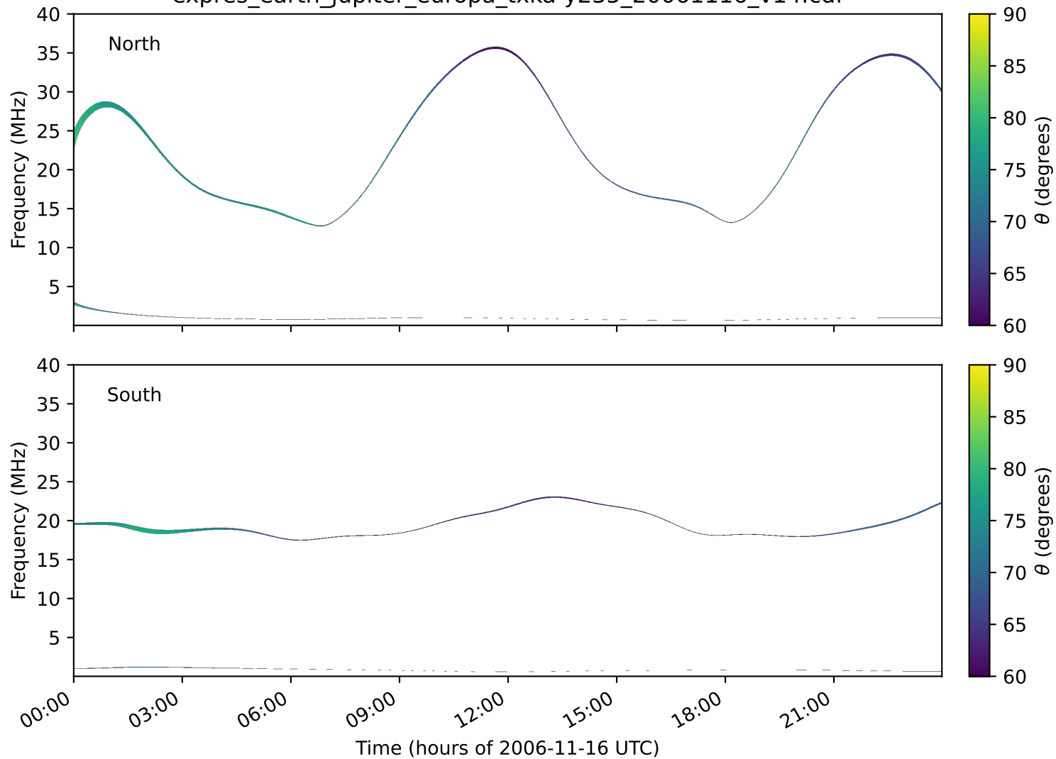
expres_earth_jupiter_europa_txka-y235_20061116_v14.cdf
