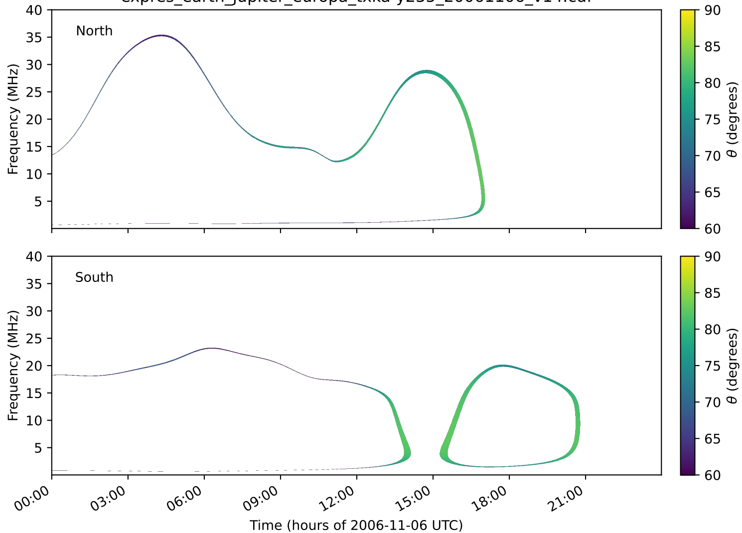
expres_earth_jupiter_europa_txka-y235_20061106_v14.cdf
