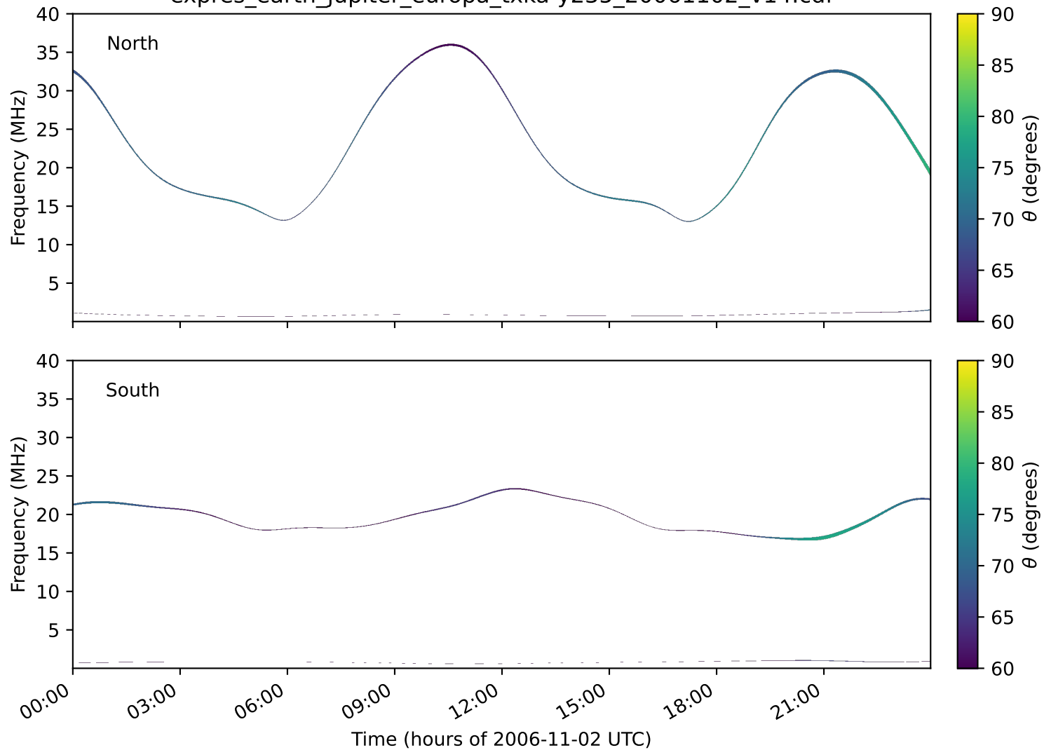
expres_earth_jupiter_europa_txka-y235_20061102_v14.cdf
