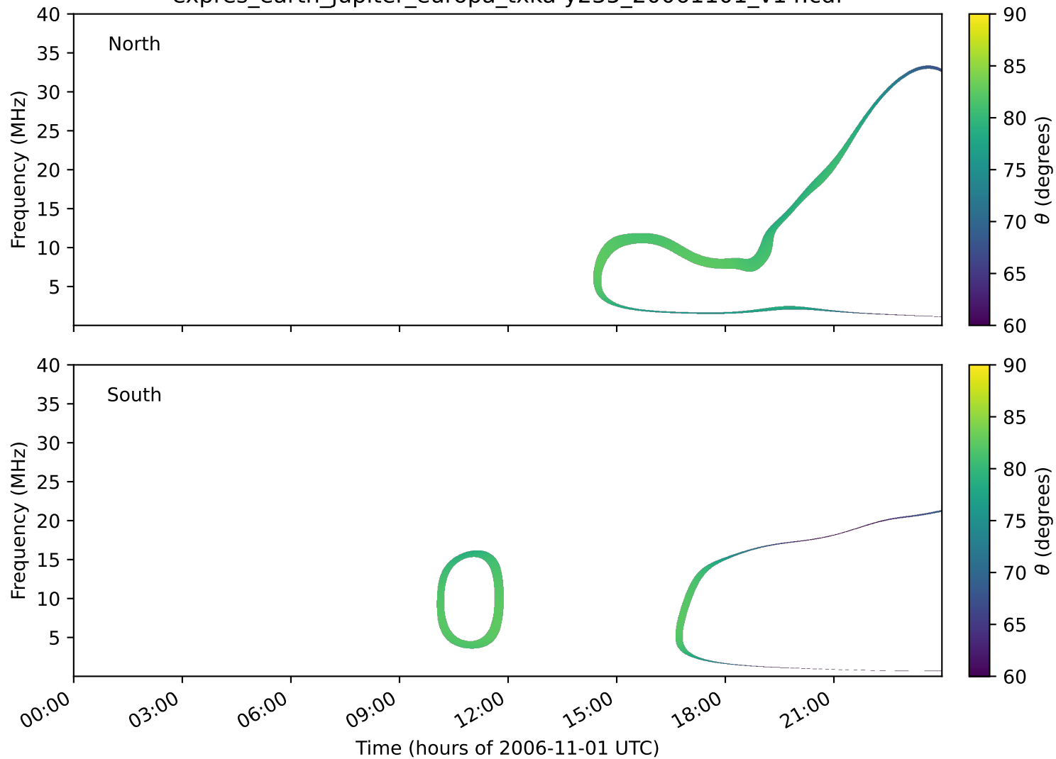
expres_earth_jupiter_europa_txka-y235_20061101_v14.cdf
