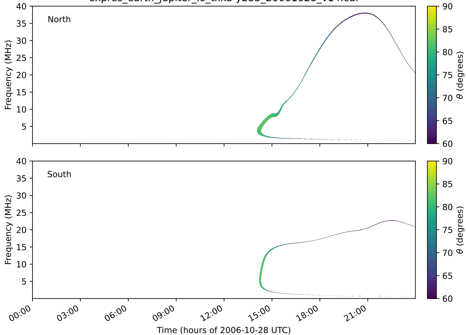
expres_earth_jupiter_io_txka-y235_20061028_v14.cdf
