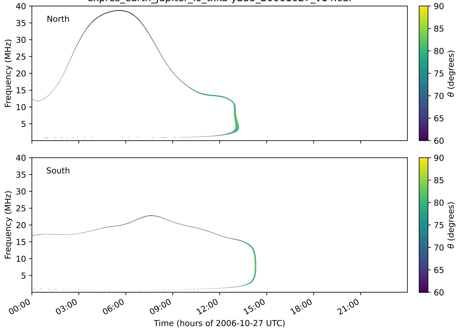
expres_earth_jupiter_io_txka-y235_20061027_v14.cdf
