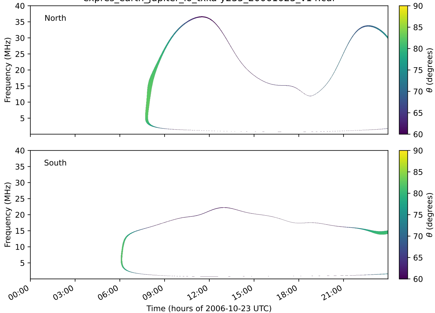
expres_earth_jupiter_io_txka-y235_20061023_v14.cdf
