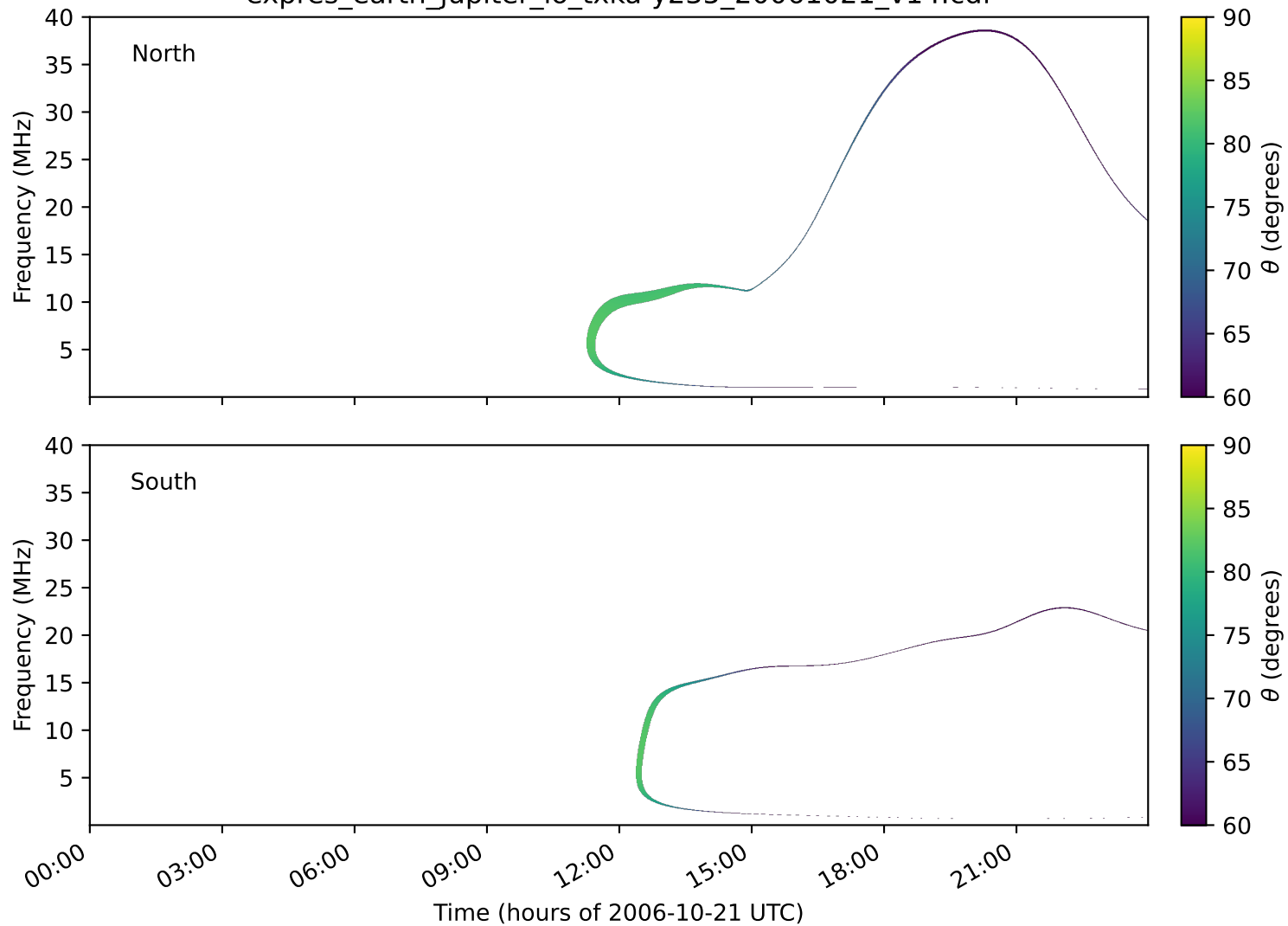
expres_earth_jupiter_io_txka-y235_20061021_v14.cdf
