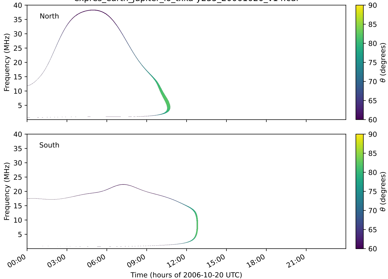
expres_earth_jupiter_io_txka-y235_20061020_v14.cdf
