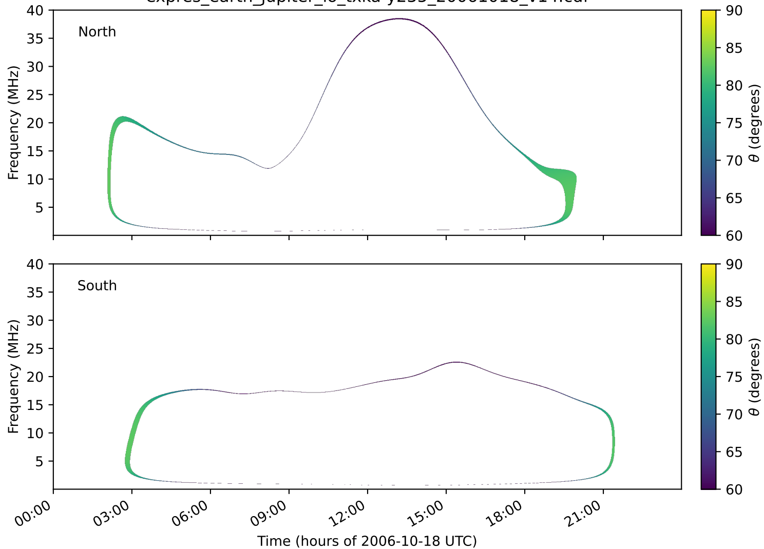
expres_earth_jupiter_io_txka-y235_20061018_v14.cdf
