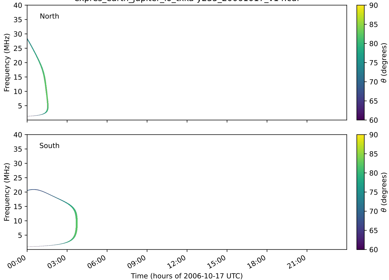
expres_earth_jupiter_io_txka-y235_20061017_v14.cdf
