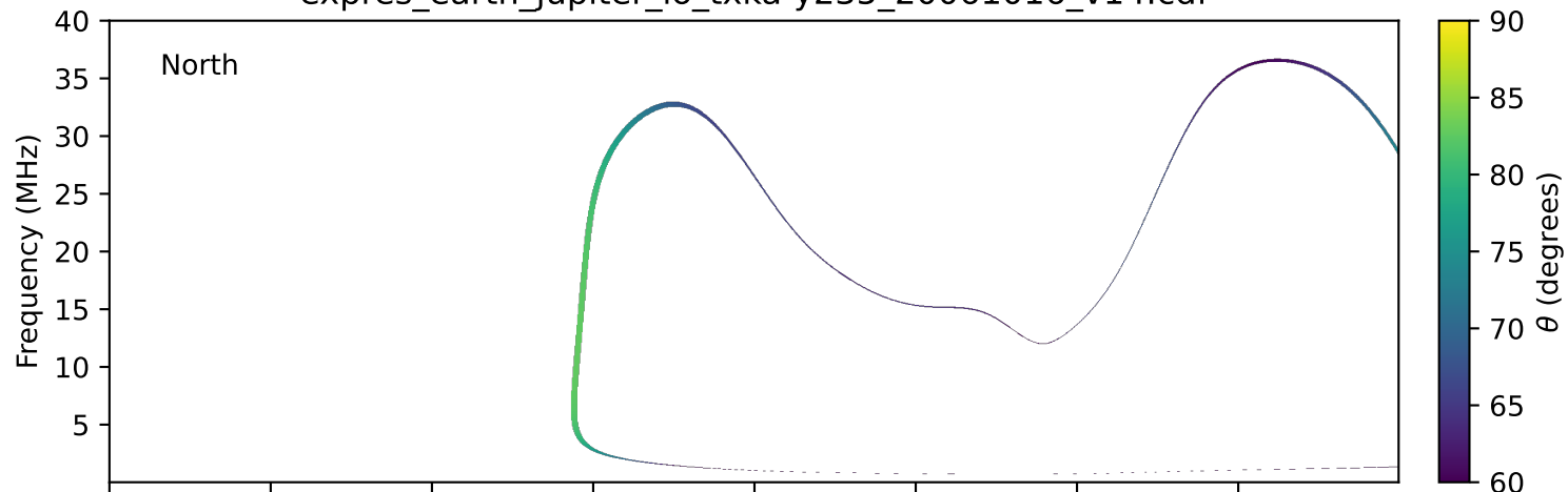
expres_earth_jupiter_io_txka-y235_20061016_v14.cdf
