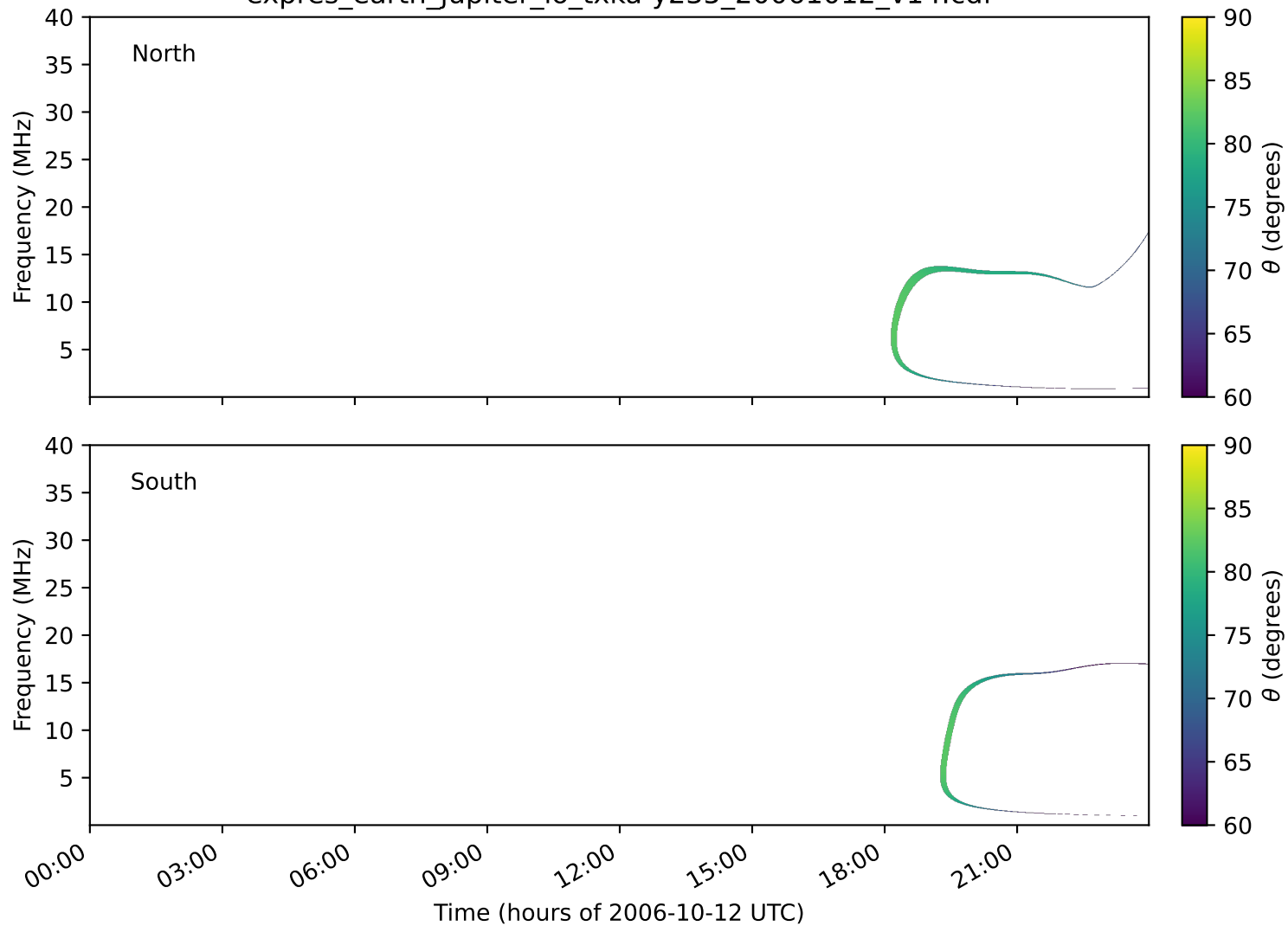
expres_earth_jupiter_io_txka-y235_20061012_v14.cdf
