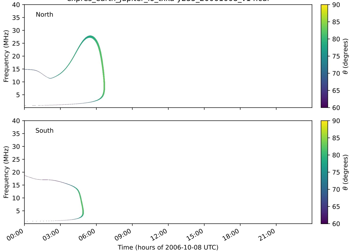
expres_earth_jupiter_io_txka-y235_20061008_v14.cdf
