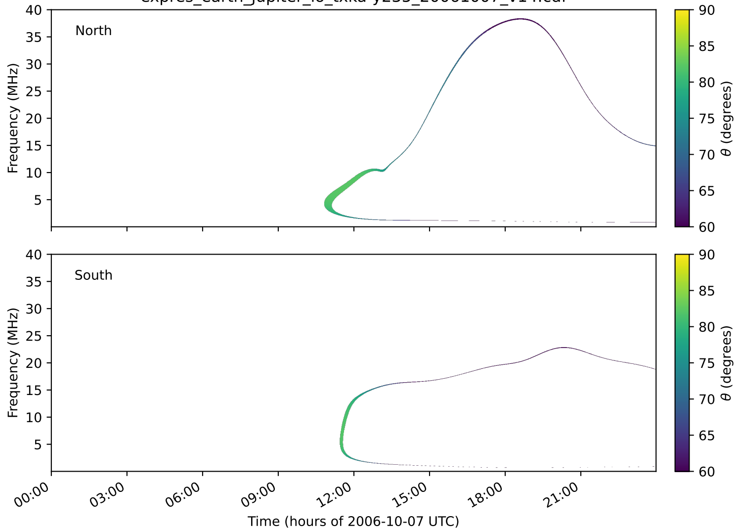
expres_earth_jupiter_io_txka-y235_20061007_v14.cdf
