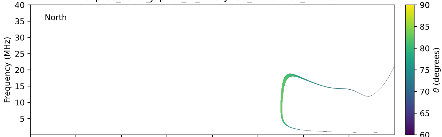
expres_earth_jupiter_io_txka-y235_20061005_v14.cdf
