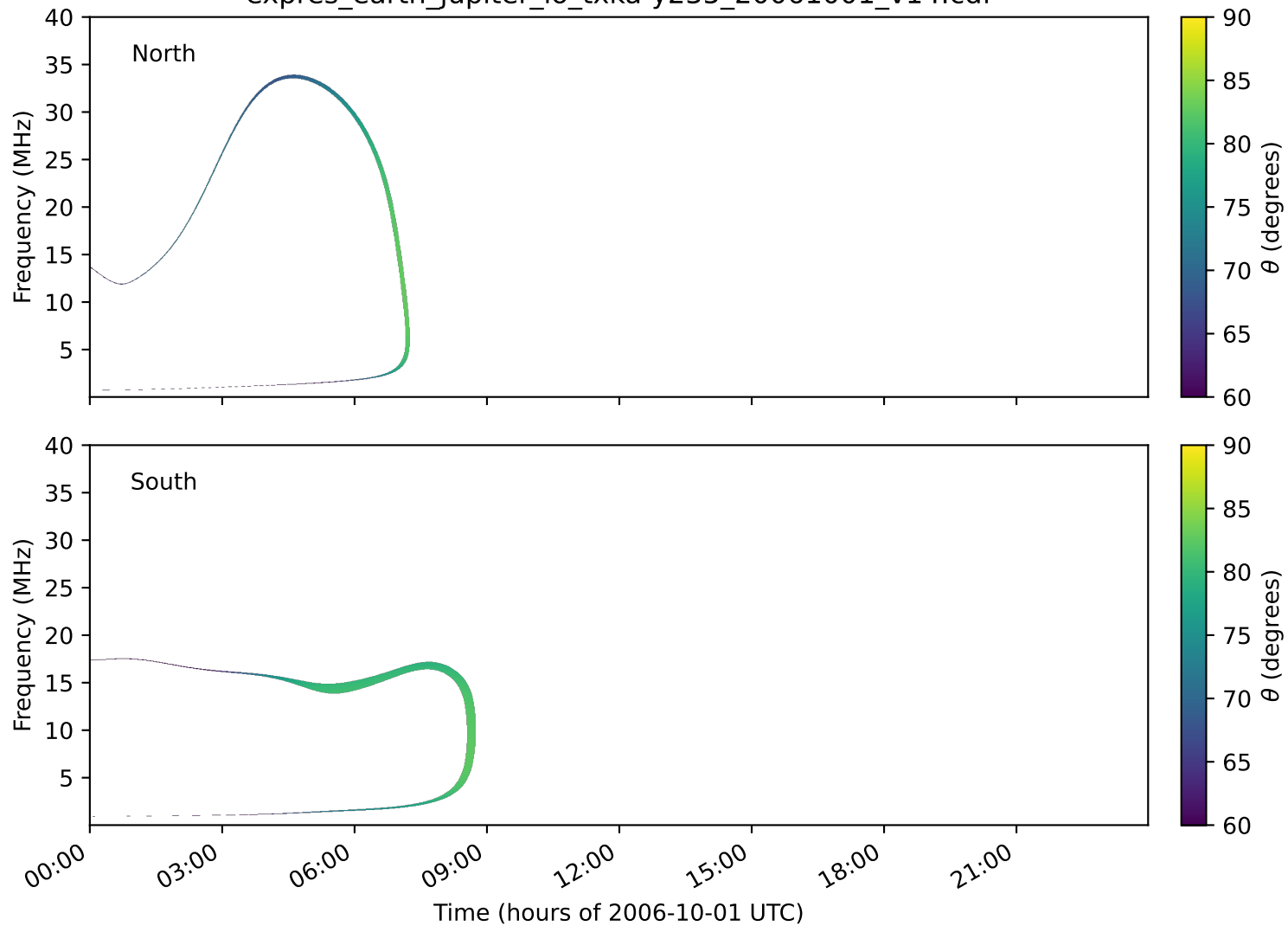
expres_earth_jupiter_io_txka-y235_20061001_v14.cdf
