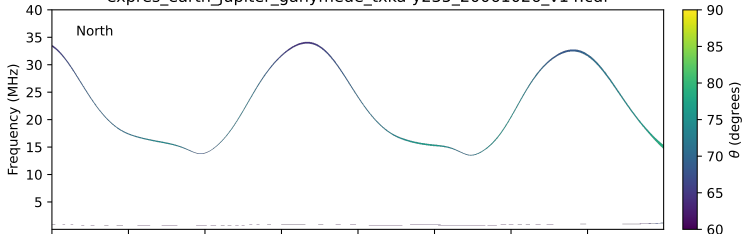
expres_earth_jupiter_ganymede_txka-y235_20061026_v14.cdf
