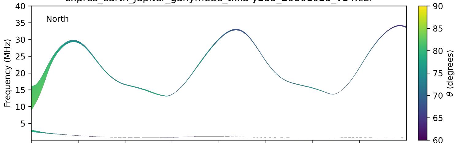
expres_earth_jupiter_ganymede_txka-y235_20061025_v14.cdf
