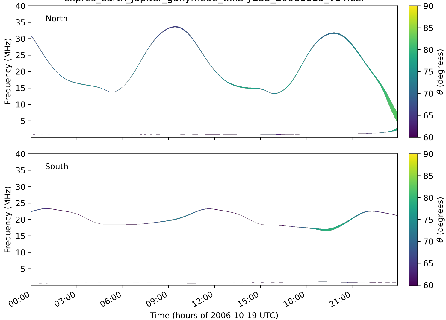
expres_earth_jupiter_ganymede_txka-y235_20061019_v14.cdf
