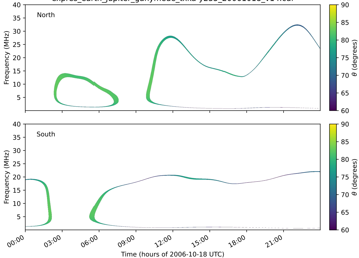
expres_earth_jupiter_ganymede_txka-y235_20061018_v14.cdf
