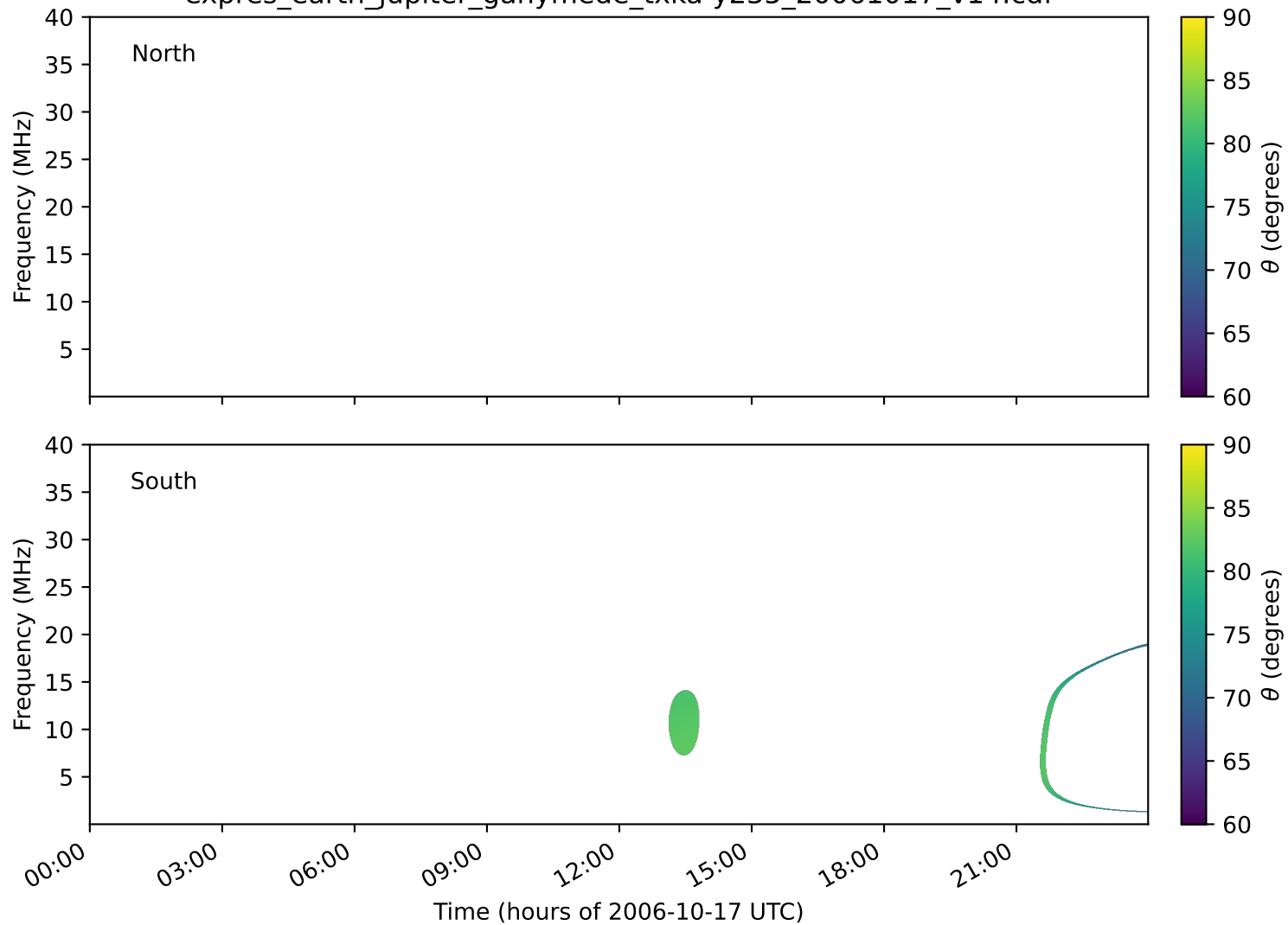
expres_earth_jupiter_ganymede_txka-y235_20061017_v14.cdf
