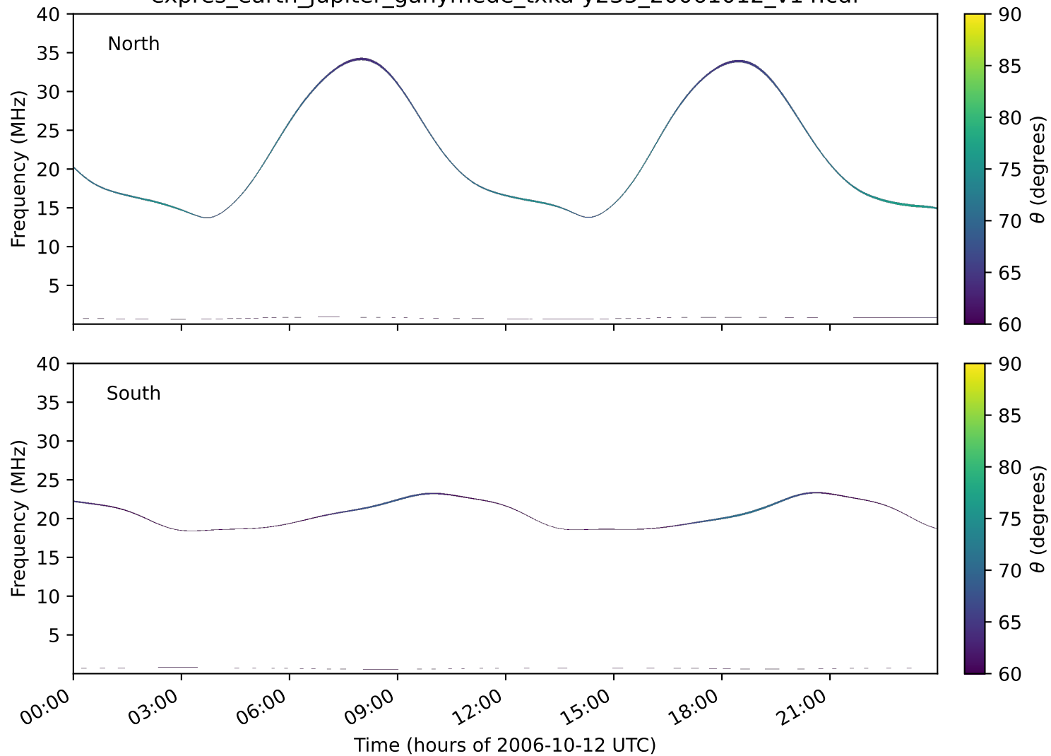
expres_earth_jupiter_ganymede_txka-y235_20061012_v14.cdf
