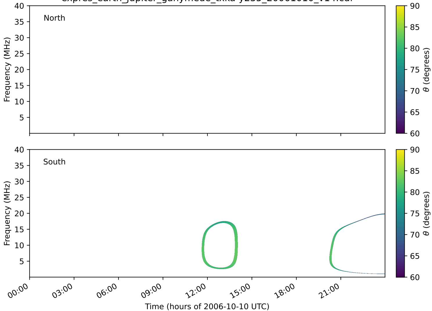
expres_earth_jupiter_ganymede_txka-y235_20061010_v14.cdf
