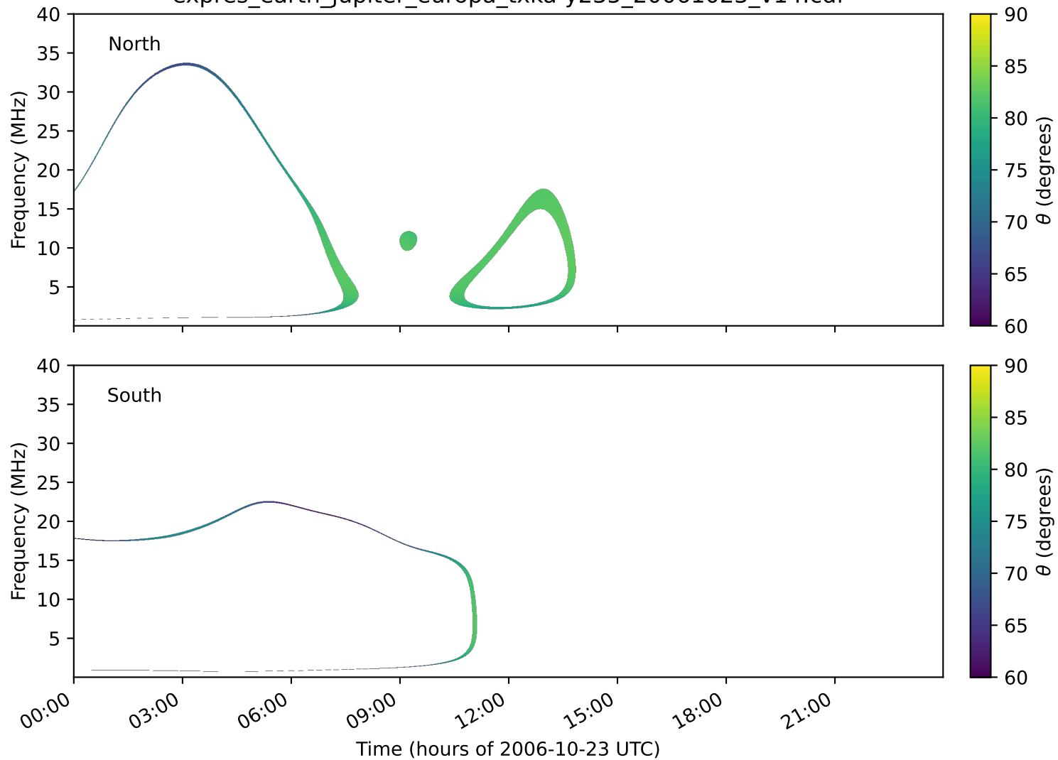
expres_earth_jupiter_europa_txka-y235_20061023_v14.cdf
