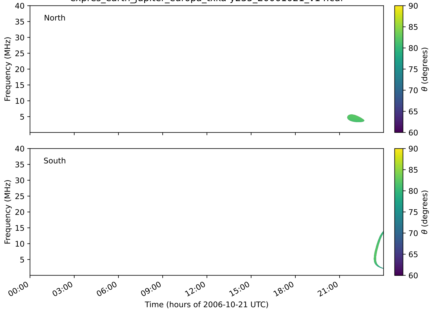
expres_earth_jupiter_europa_txka-y235_20061021_v14.cdf
