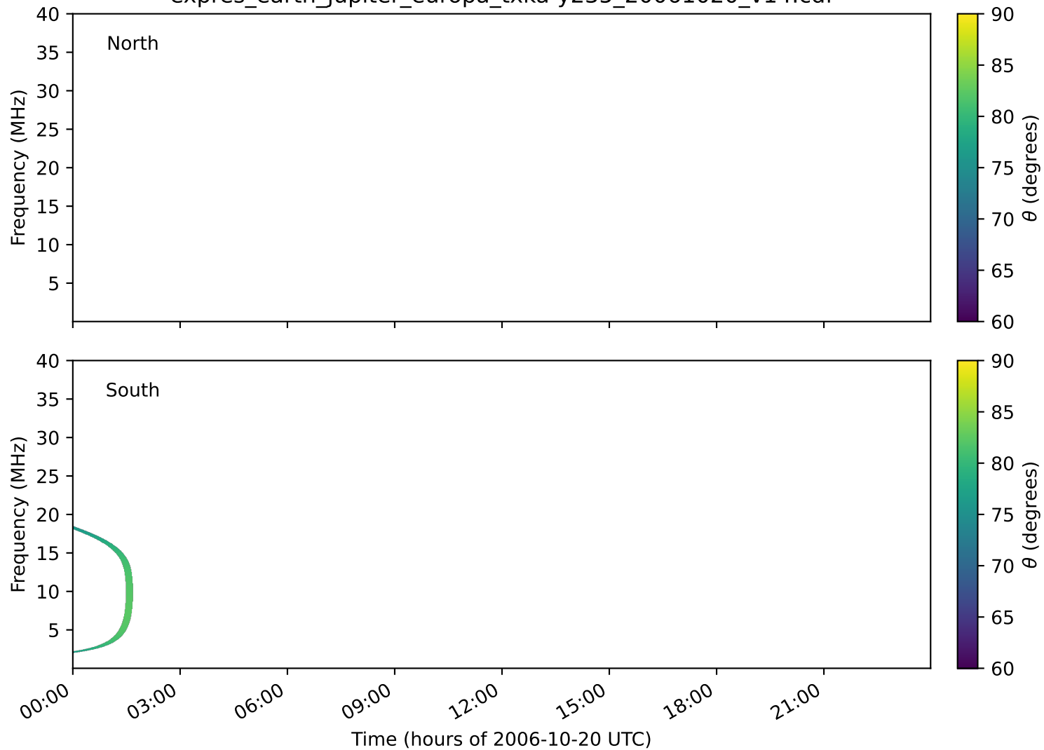
expres_earth_jupiter_europa_txka-y235_20061020_v14.cdf
